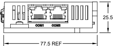
RIGHT VIEW
