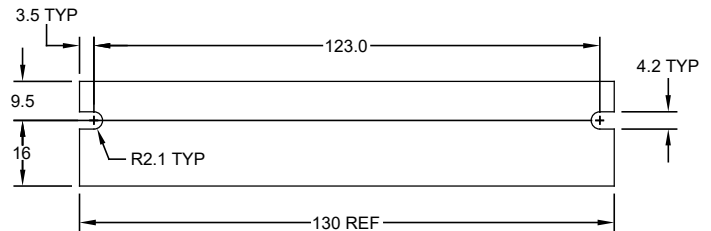
REAR VIEW
