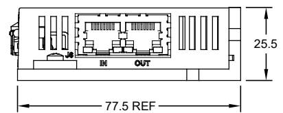
RIGHT VIEW
