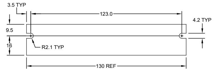
REAR VIEW
